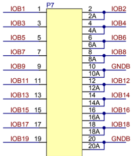
20 way triple Row RA + BOX
